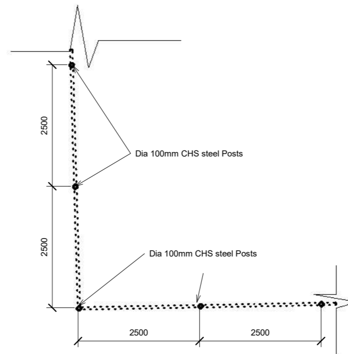
FENCE PLAN
