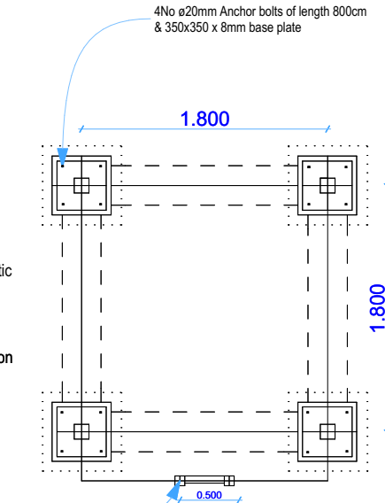
FOUNDATION PLAN Scale 1:25
