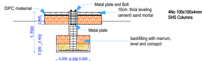
Foundation section
