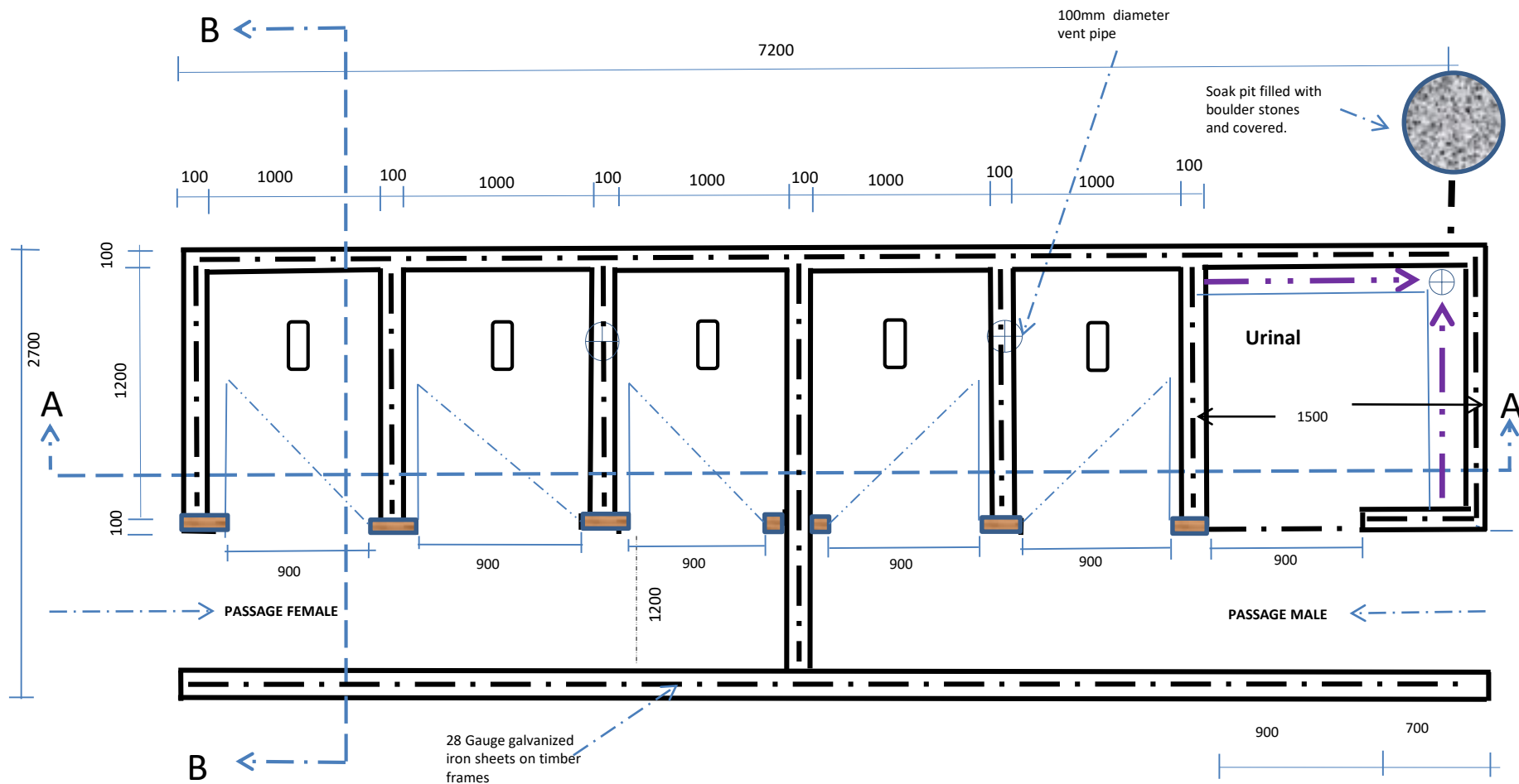
TOILET PLAN VIEW
