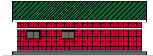
REAR ELEVATION
