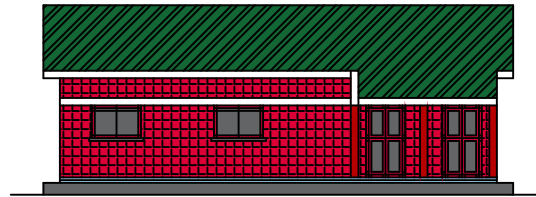
FRONT ELEVATION
