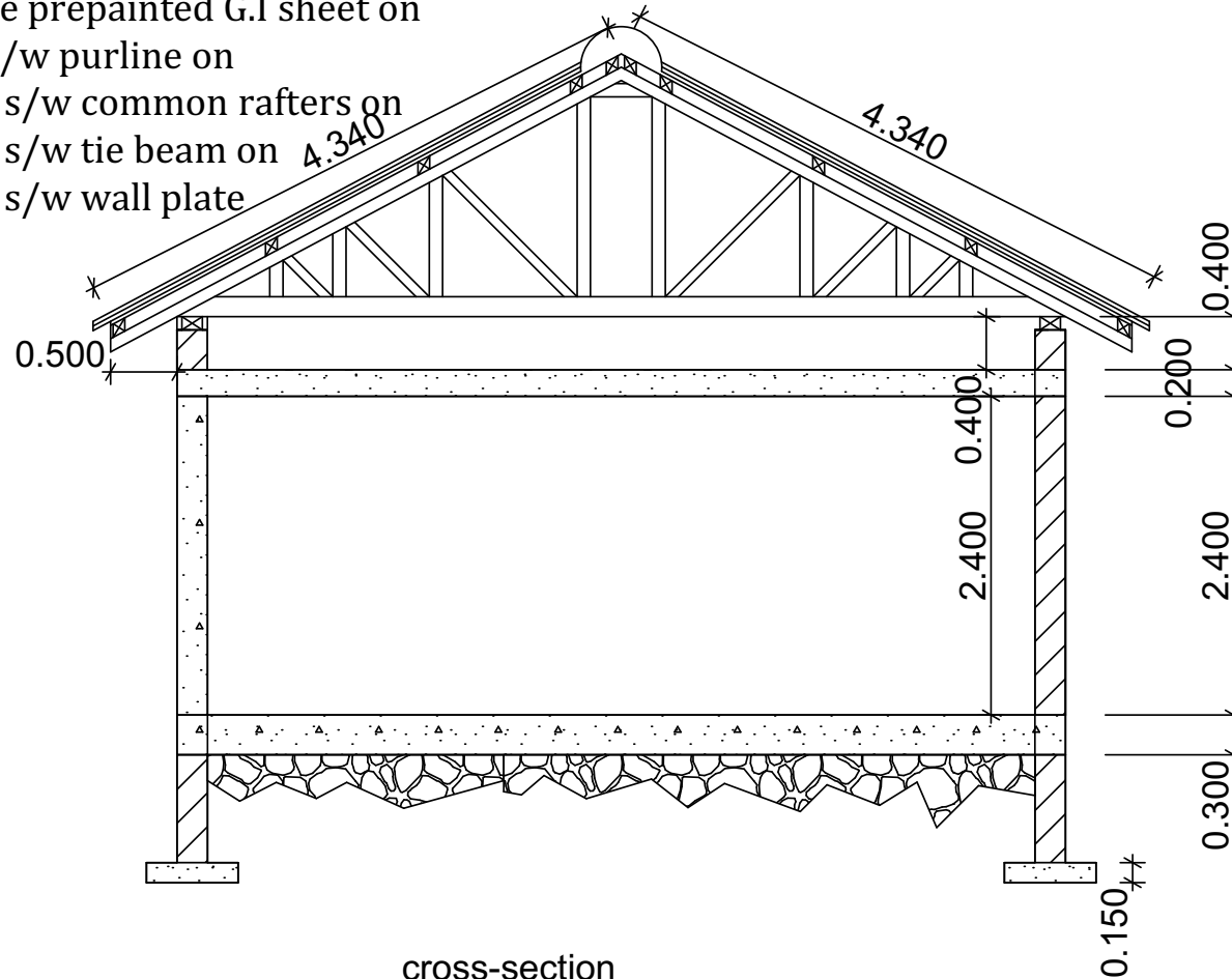
CROSS-SECTION FOR NUTRITION SITE IN KAPOETA MISSION HOSPITAL
