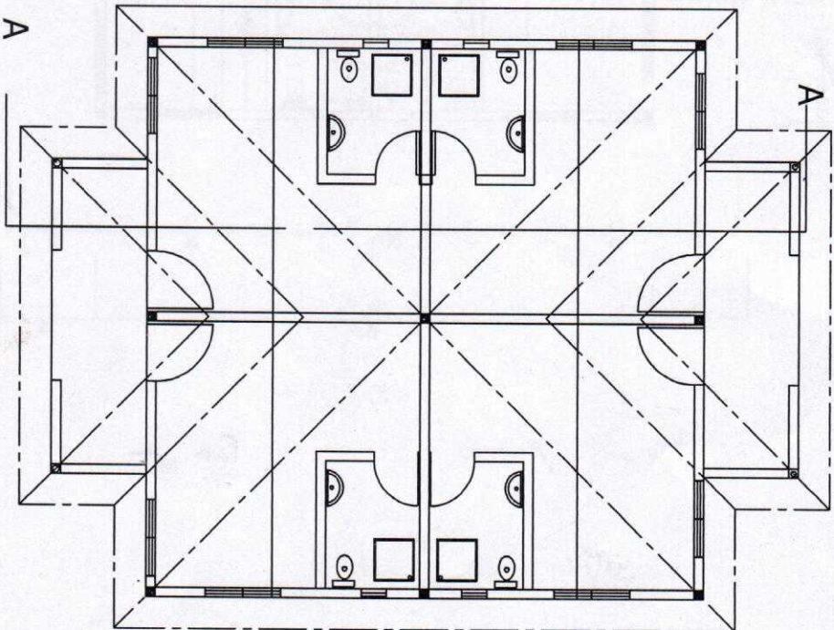
ROOFING PLAN
