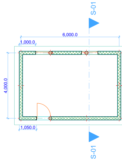
Plan View
