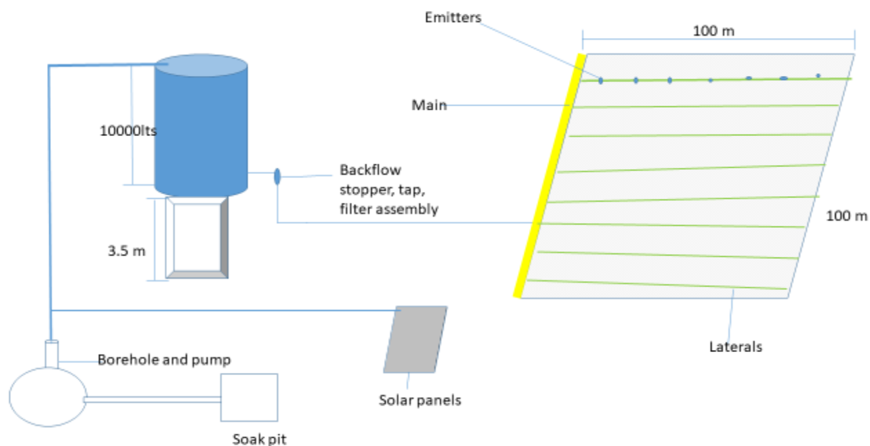
Drip Irrigation design and Layout for Gorom
