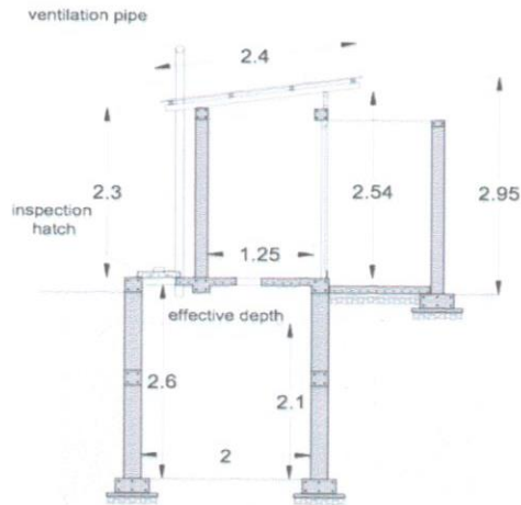
TRANSVERSAL SECTION
