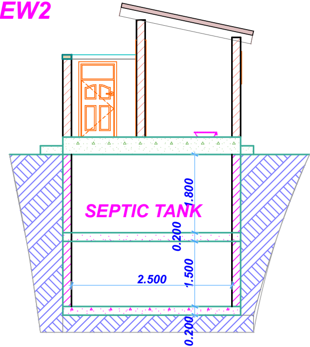
X-SECTION THROUGH SEPTIC TANK
