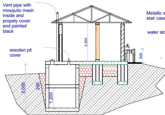
CROSS-SECTION X-X
