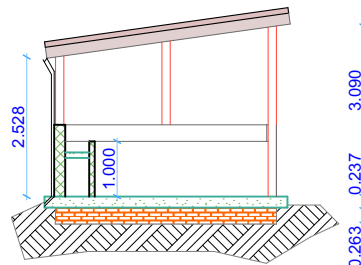
Section S-01
