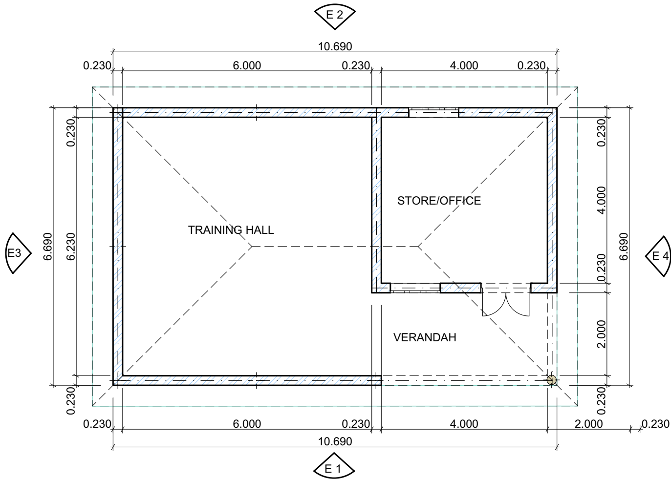
GROUND PLAN FOR NUTRITION SITE IN KAPOETA MISSION HOSPITAL
