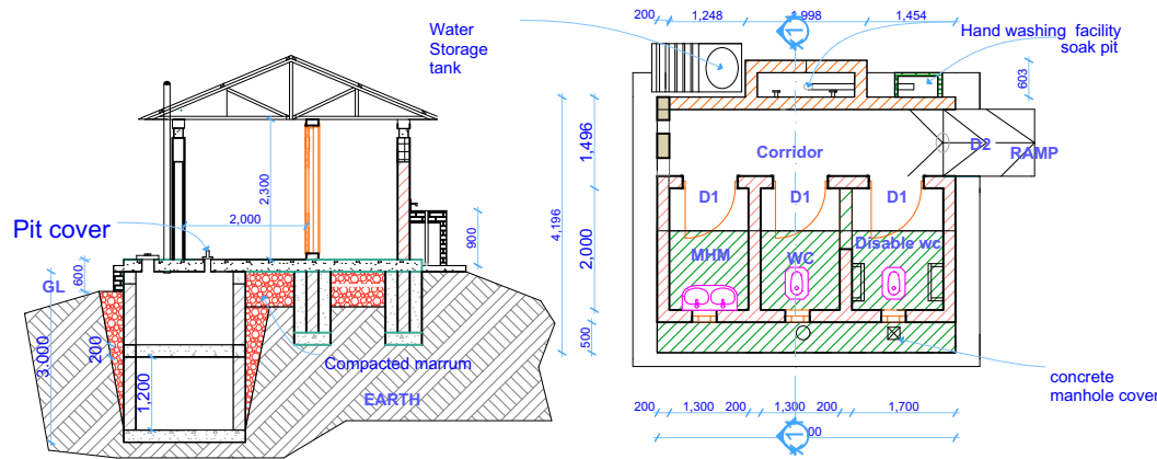
PLAN
